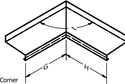
Internal Corner
